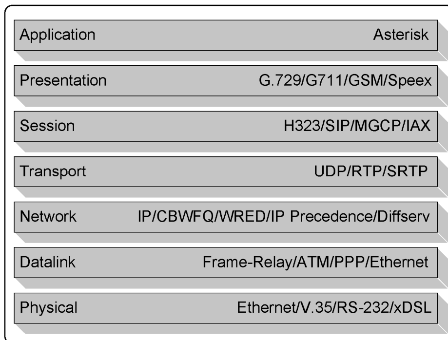
Figure 5.3 VoIP in the OSI model.
