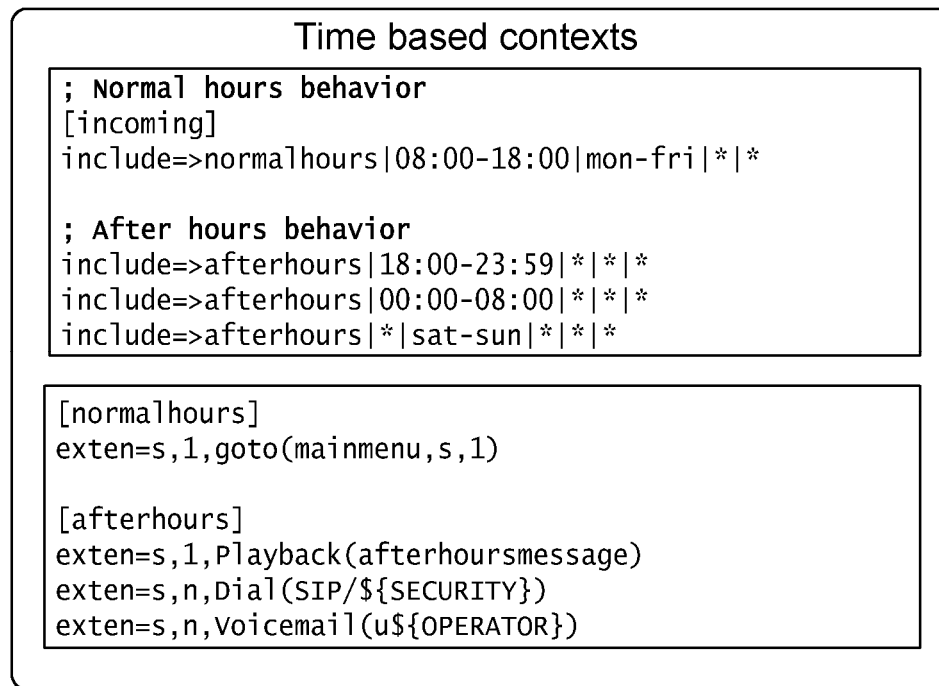
Figure 9.18 Time based contexts
