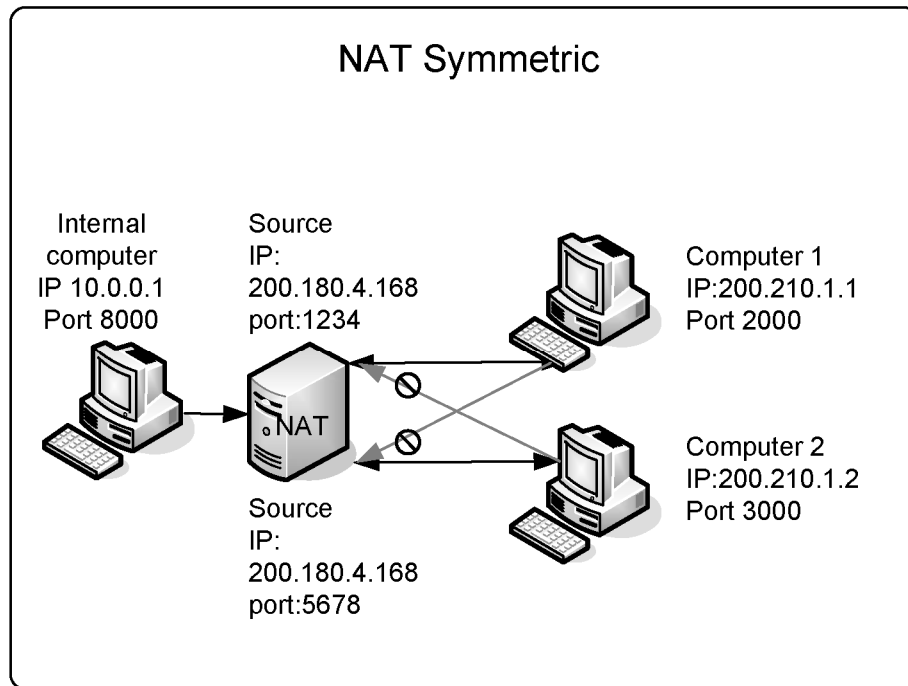
Figure 7.13 NAT Symmetric
