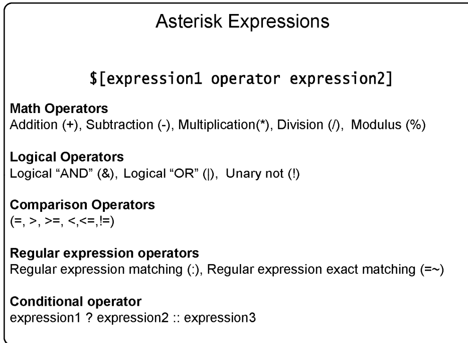
Figure 8.5 Asterisk expressions
