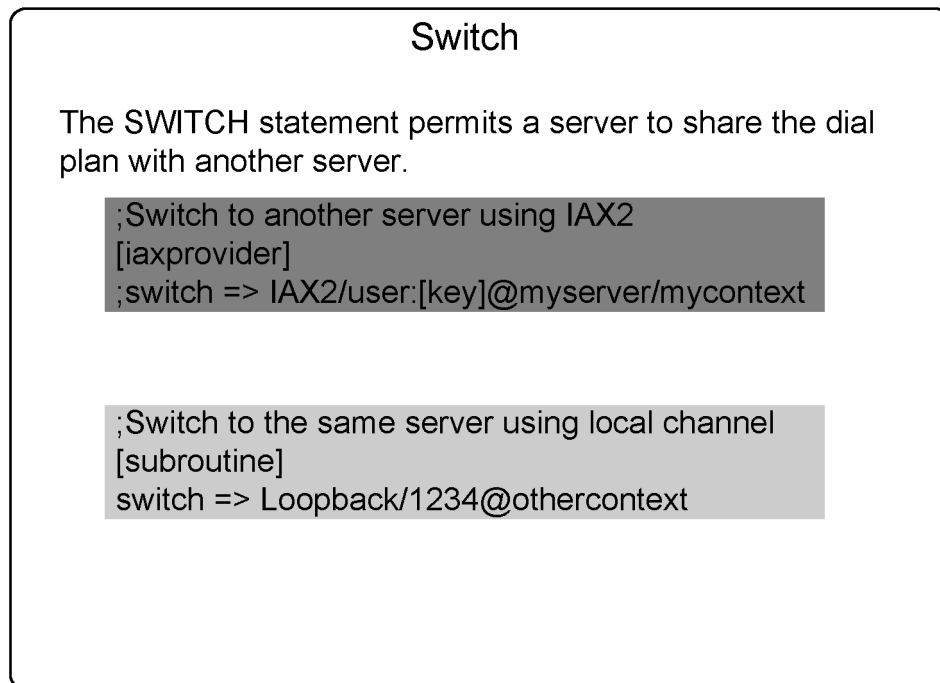
Figure 9.12 Switch statement
