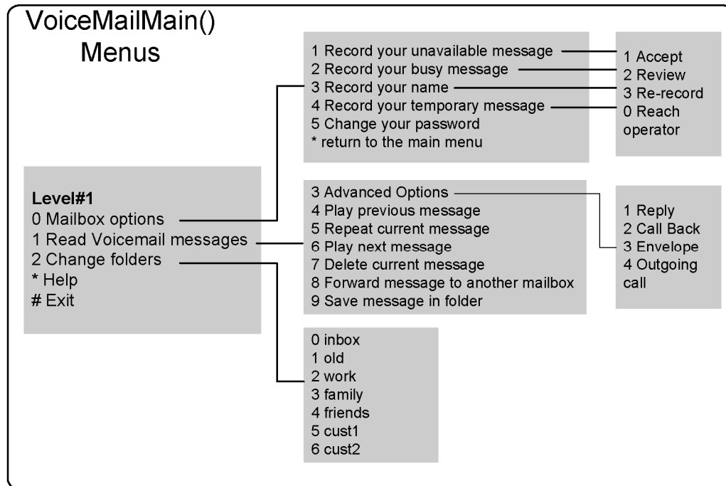
Figure 12.5 Voicemailmain menu
