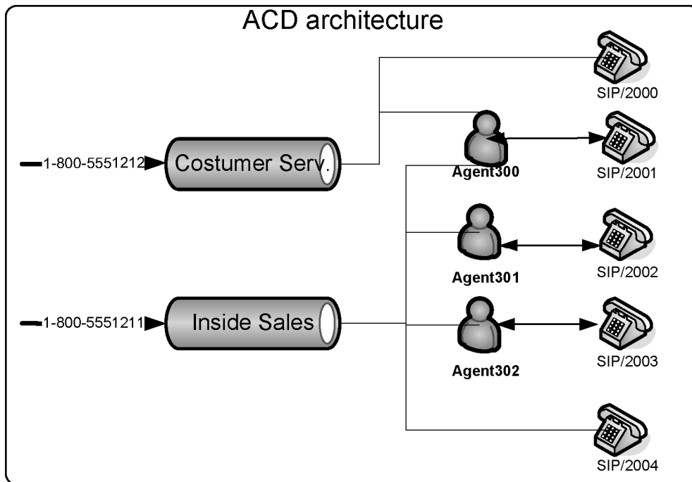
Figure 11.3 ACD architecture
