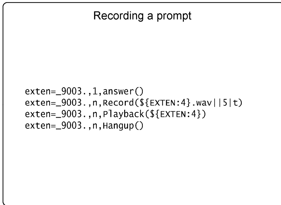
Figure 9.8 Recording a prompt()
