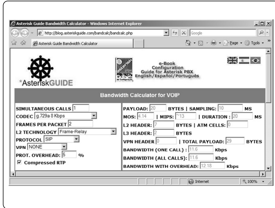
Figure 5.10 VoIP bandwidth using cRTP
