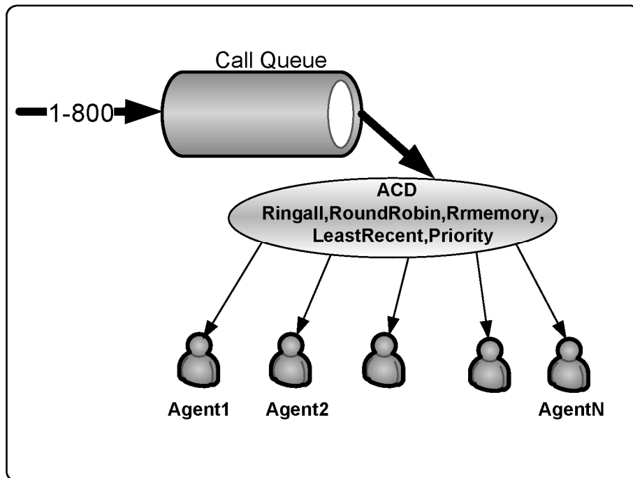
Figure 11.2 Automatic Call Distribution
