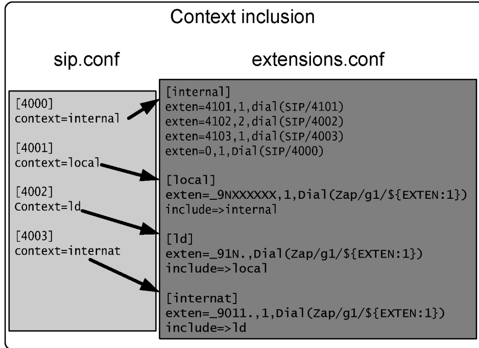
Figure 9.11 Context inclusion
