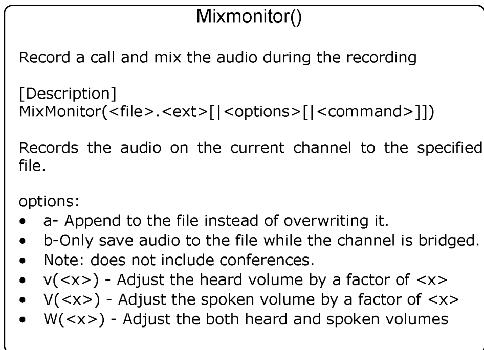
Figure 10.9 Mixmonitor application
