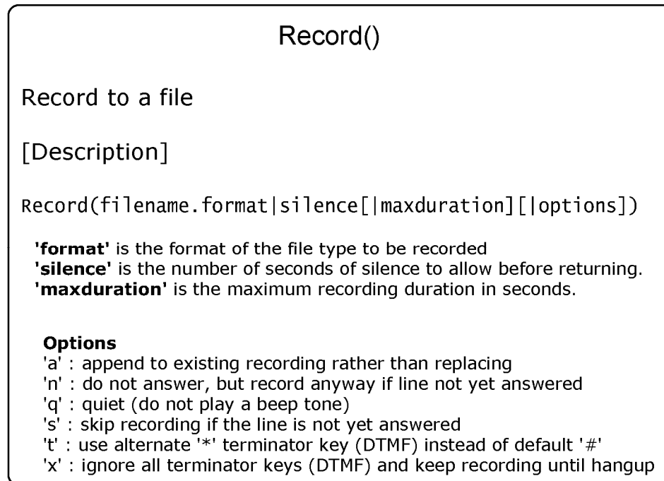
Figure 9.4 Record() application
