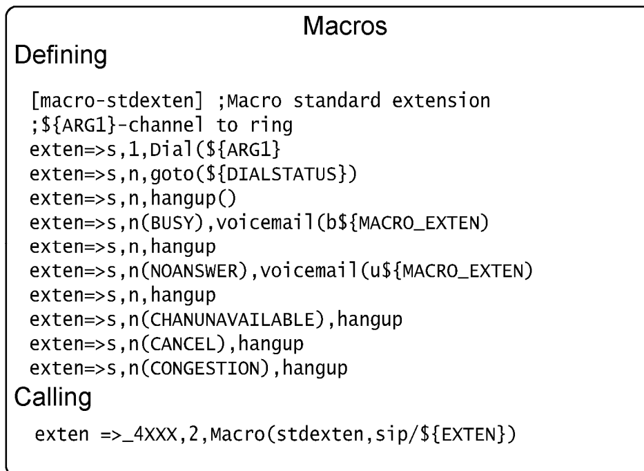
Figure 9.14 Macros
