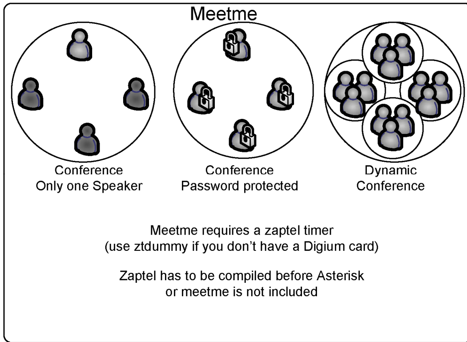
Figure 10.7 meetme application
