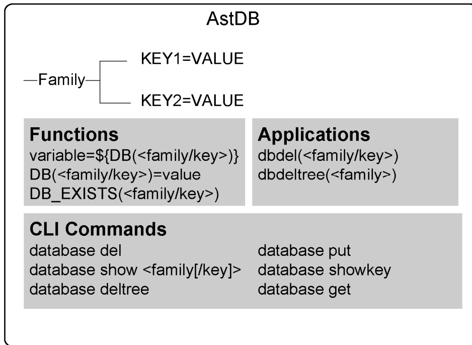
Figure 9.15 Asterisk DB
