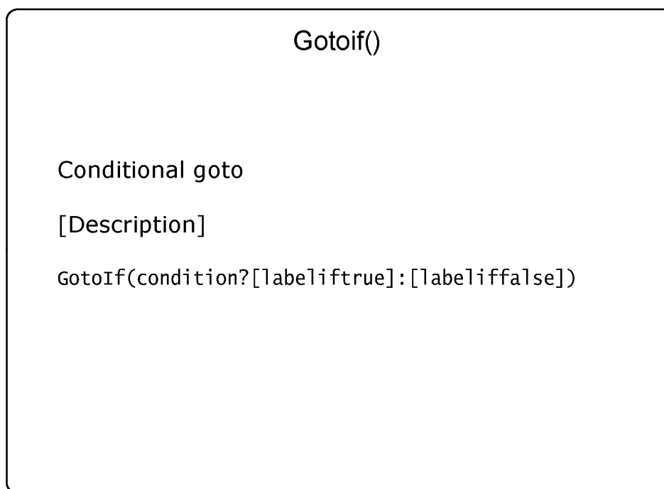
Figure 9.7 Gotoif() application
