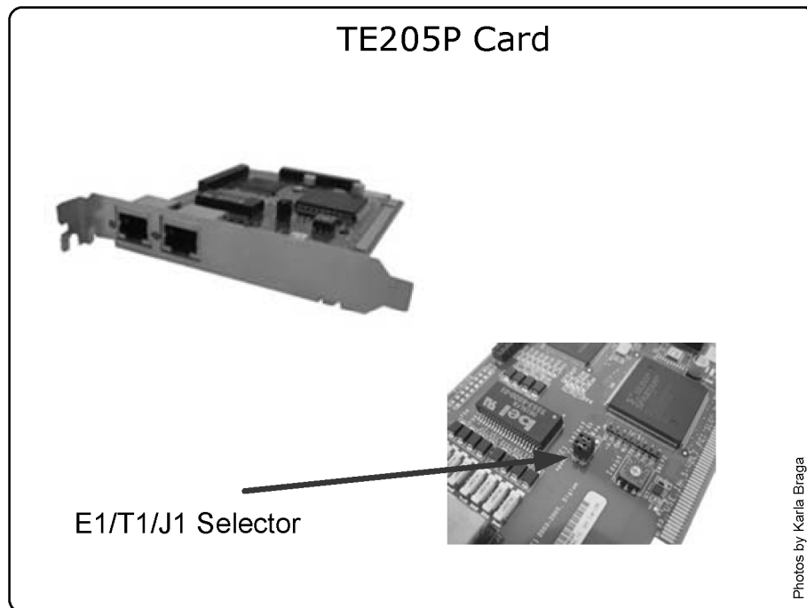
Figure 4.8 TE205P Card
