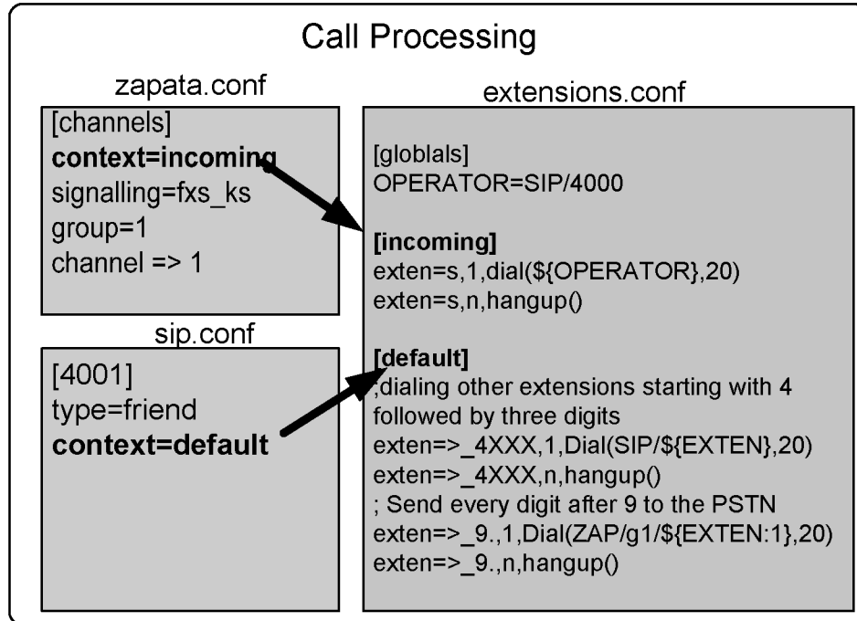
Figure 8.4 Basic Dial Plan
