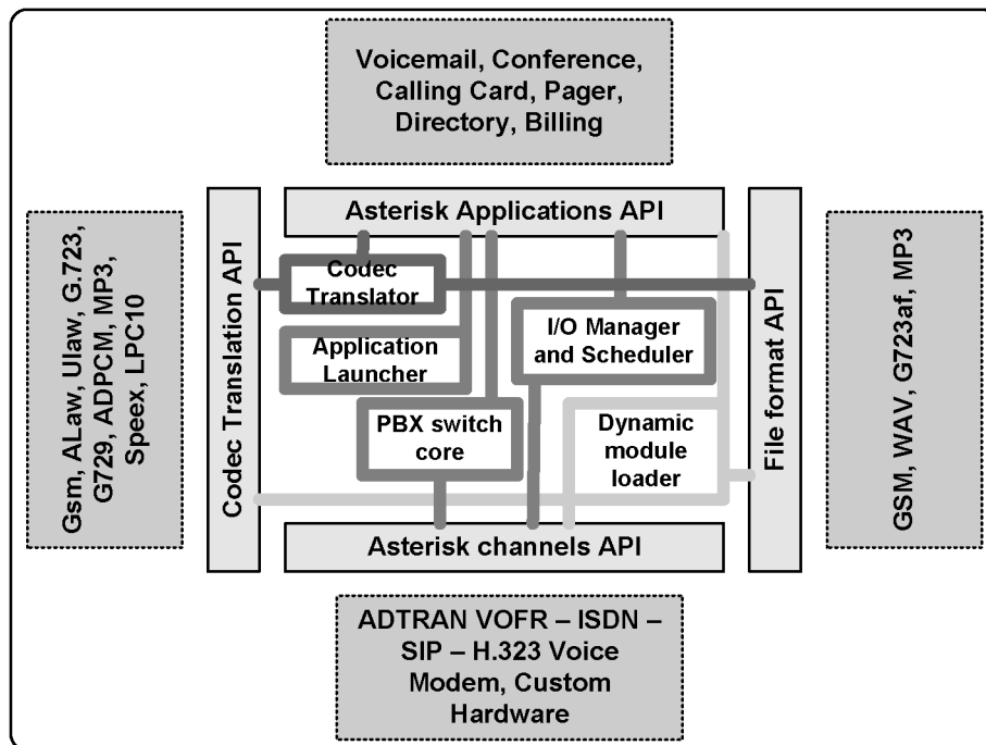
Figure 1.1 - Asterisk Architecture.
