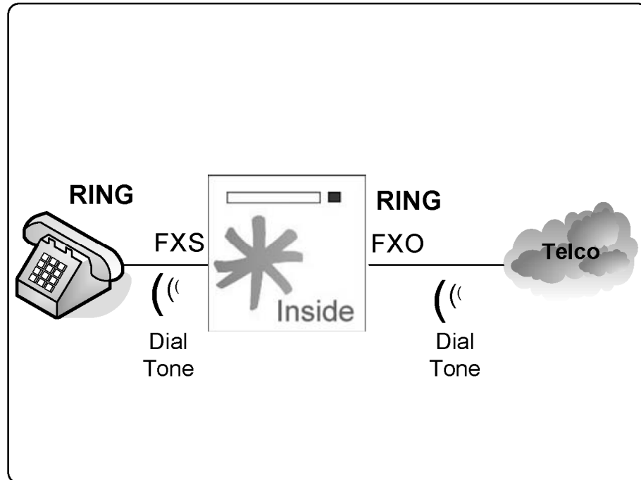
Figure 3.1 FXO and FXS Interfaces
