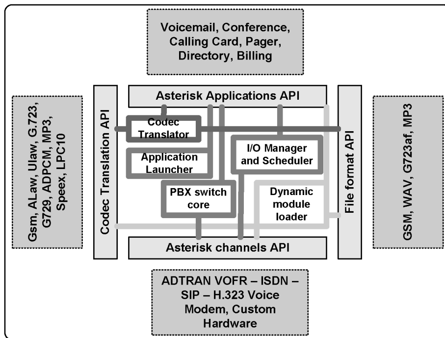
Figure 5-2 Asterisk architecture
