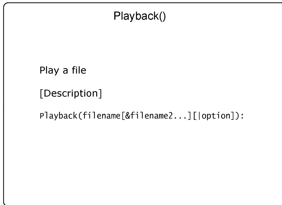
Figure 9.5 Playback() application
