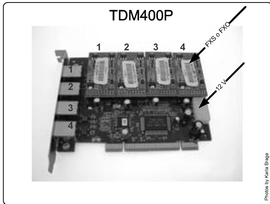
Figure 4.6 TDM400 card
