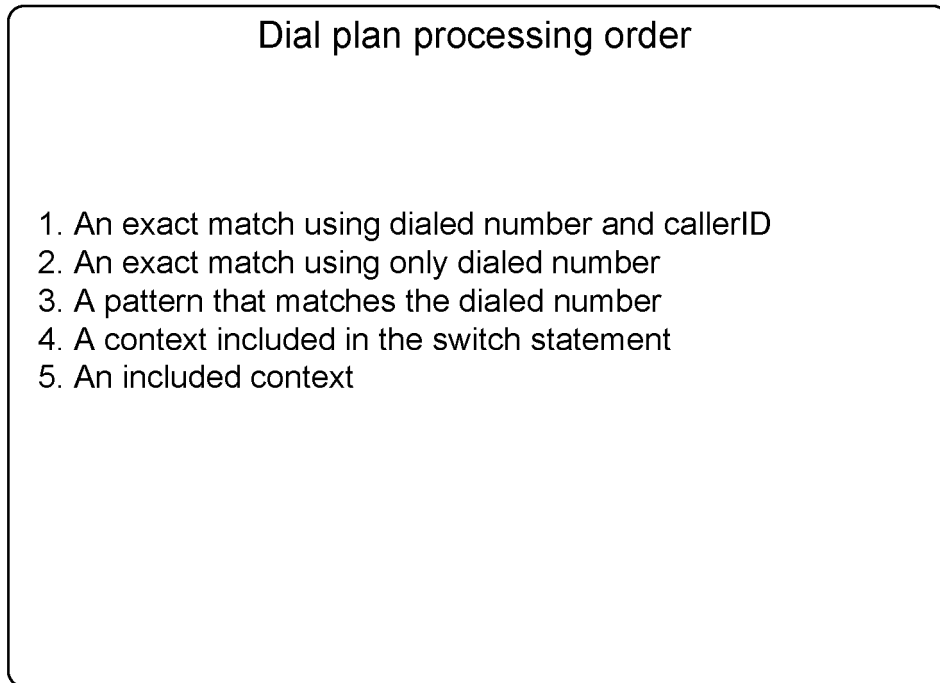
Figure 9.13 Dial plan processing order
