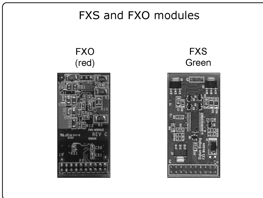
Figure 4.7 FXS Module (S100M - green), FXO module (X100M – red)
